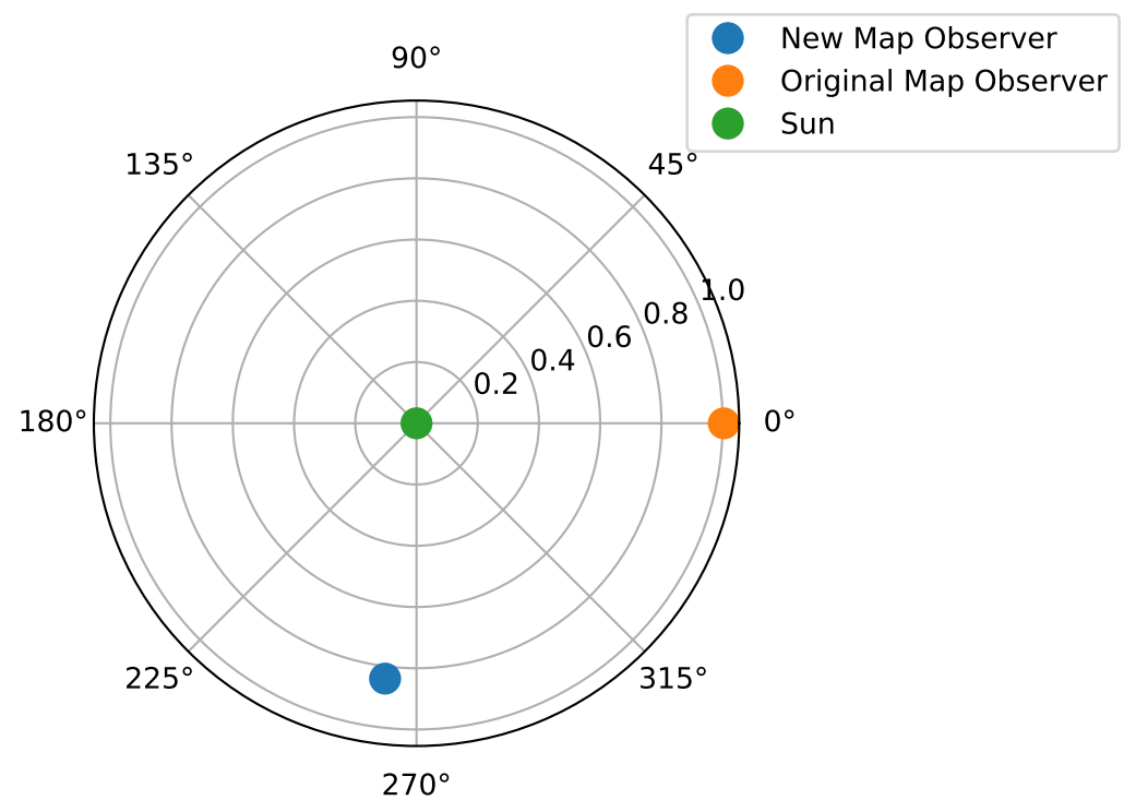
Map as seen by observer 2021-04-17T00:00:04.840
