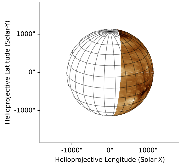
Map as seen by observer 2021-04-17T00:00:04.840
