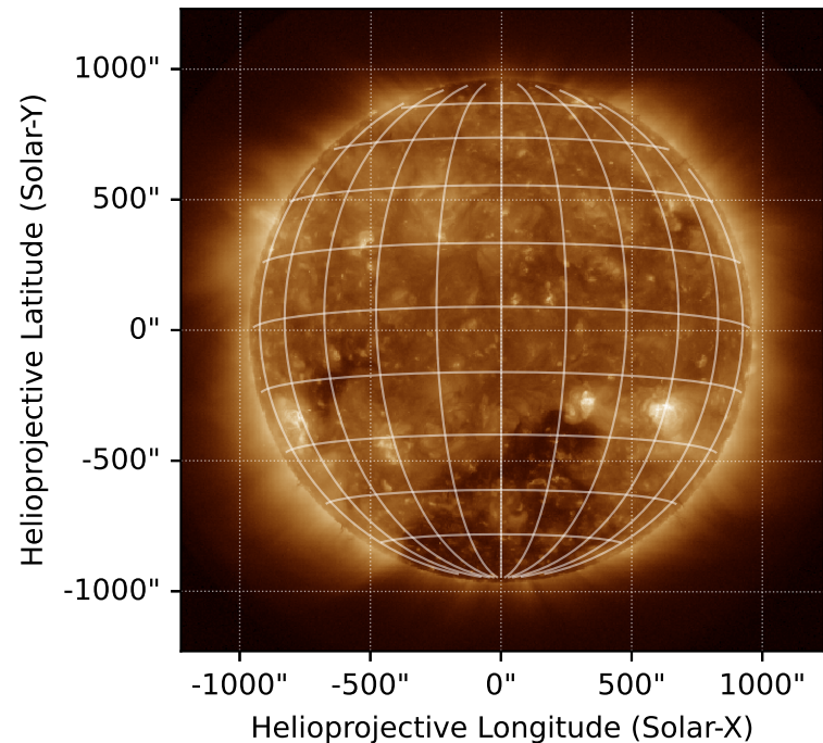
Input AIA map 2021-04-17T00:00:04.840
